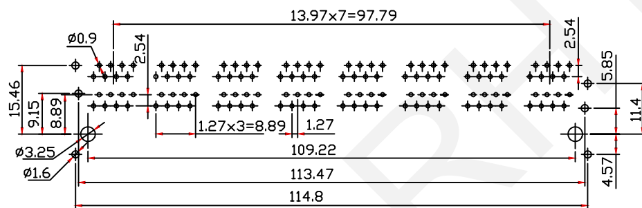
PCB Layout
